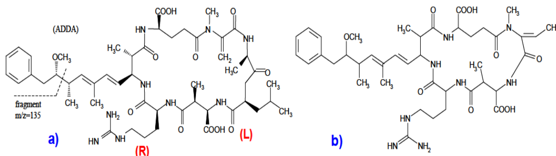
Figure 1. Structures of cyanobacterial toxins. a) Microcystin-LR. The other microcystins are derived from this by replacing the marked amino acids (L) and (R) by the amino acids indicated in their names. b) Nodularin.
