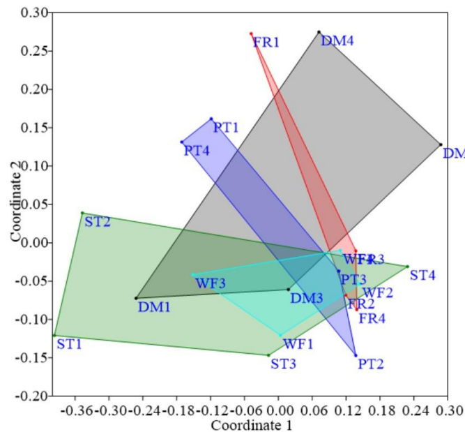
Figure 9. Non-metric dimensional scaling (NMDS) of dragonflies composition in five habitats (stress value: 0.15); ANOSIM ( R = 0.00083 ; P = 0.4597 ). (DM: dam; FR: forest; PT: plantation; ST: settlement; WF: waterfall)
