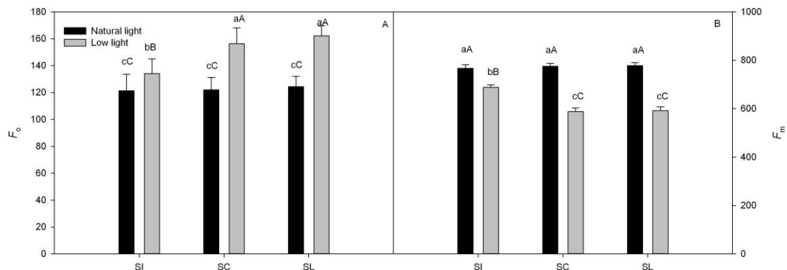
Figure 5. Minimal fluorescence ( F_0 ) and maximum fluorescence ( F_m ) in leaves of three Syringa . Data in the figure are mean \pm SD, values followed by different small letters mean significant difference ( p < 0.05 ), values followed by different capital letters mean very significant difference ( p < 0.01 ). SI: Syringa oblata Iandl; SC: Syringa chinensis ; SL: Syringa oblata var. affinis Lingelsh
