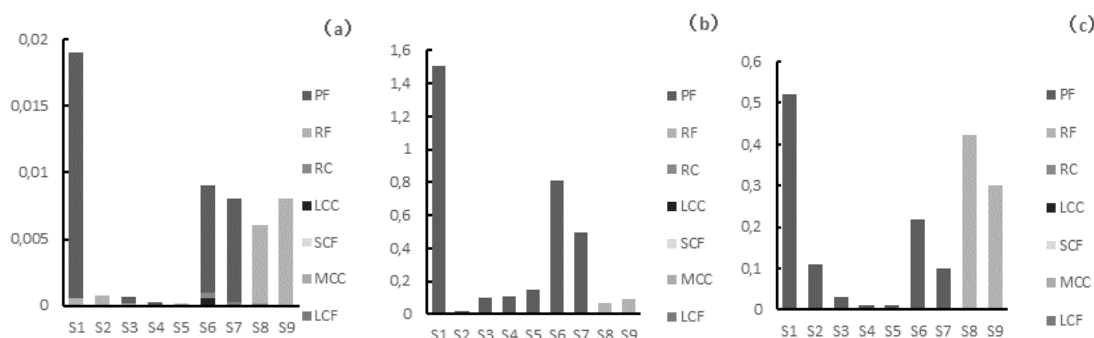
Figure 2. Spatial distribution of zooplankton groups biomass of spring (a), summer (b) and autumn (c). Protozoa filter feeders (PF), rotifer filter feeders (RF), rotifer carnivora (RC), small copepodas and cladocera filter feeders (SCF), middle copepodas and cladocera carnivore (MCC), large copepodas and cladocera carnivore (LCC) and large copepodas and cladocera filter feeders (LCF)
